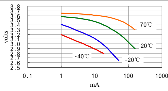
VOLTAGE VS. CURRENT
