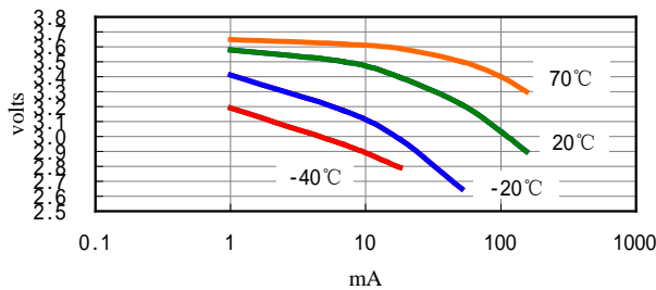
CAPACITY VS. CURRENT
