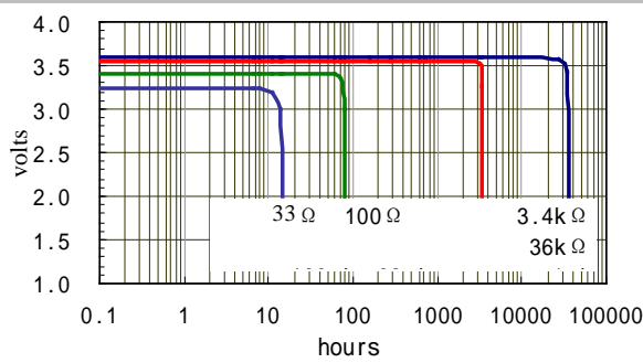
DISCHARGE CHARACTERISTICS @23±2°C
